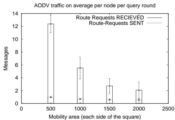
Figure 5: The major cost of running AODV at each node per query-group is RREQ messages. (Error bars indicate standard deviations.)
