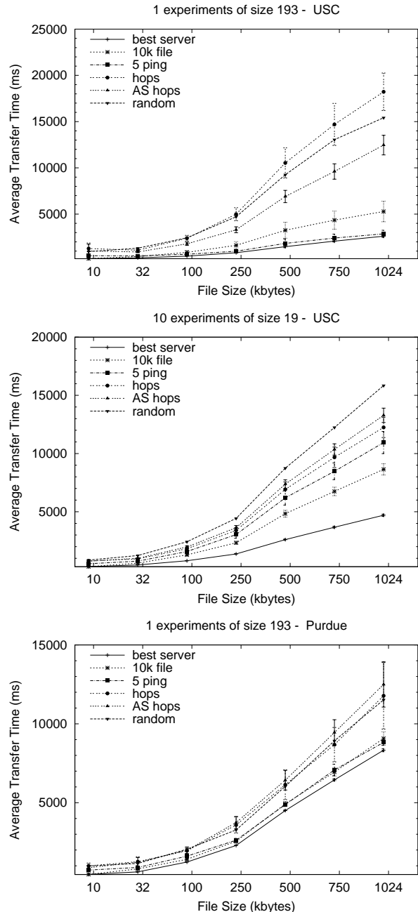
Figure 2. Performance of server selection metrics (top: USC, 193-set; middle: USC, 19-subset; bottom: Purdue, 193-set).
