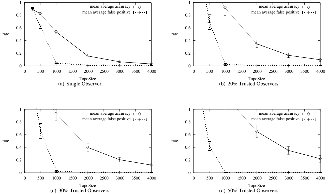
Figure 3: Accuracy rates for various percentages of observers, Group moving in Unison
