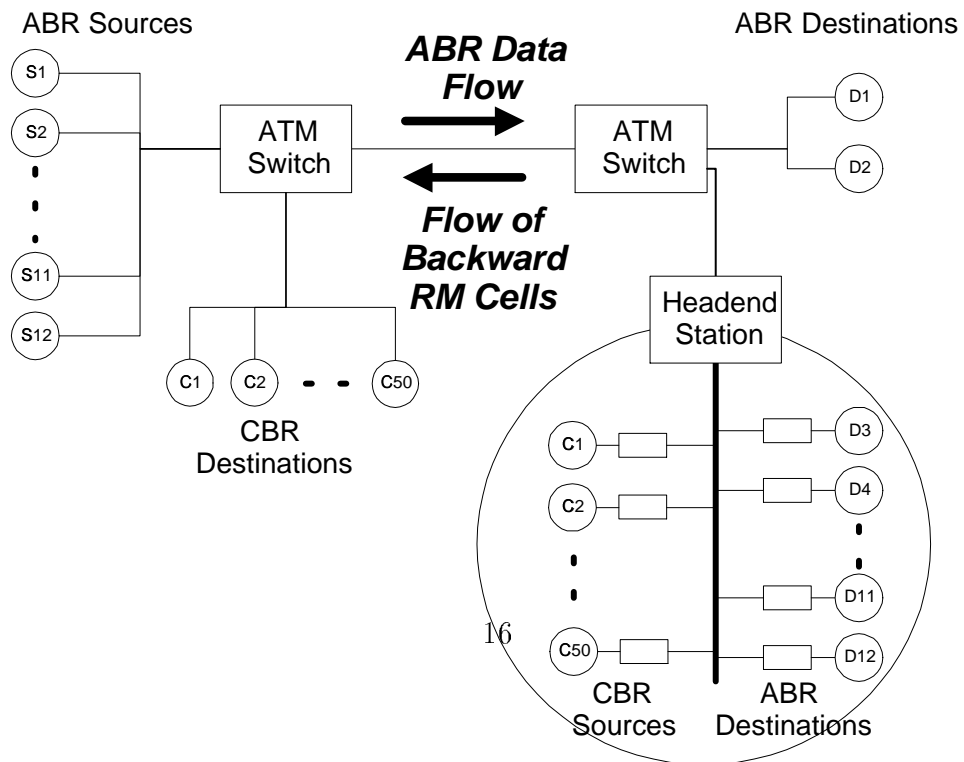
Figure 2.4: Downstream Configuration.
