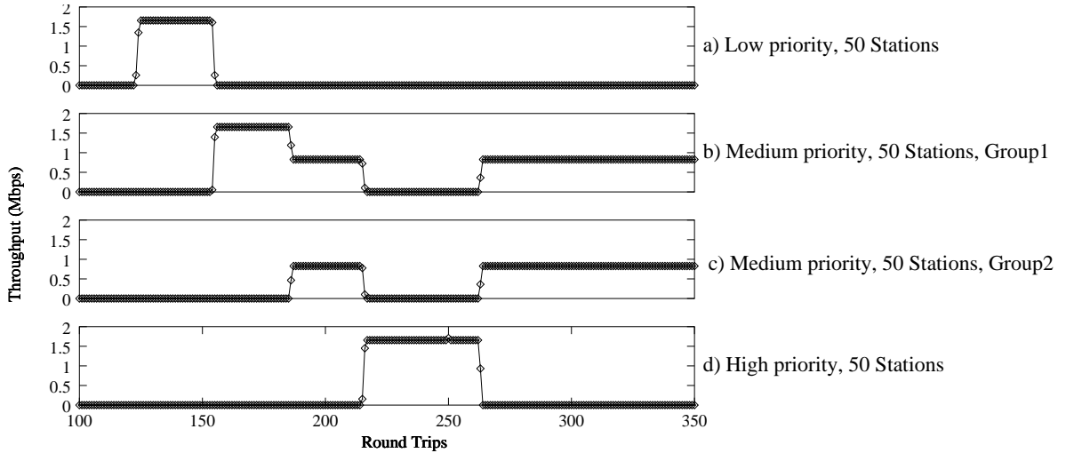
Figure 3.8: Transient Throughput
