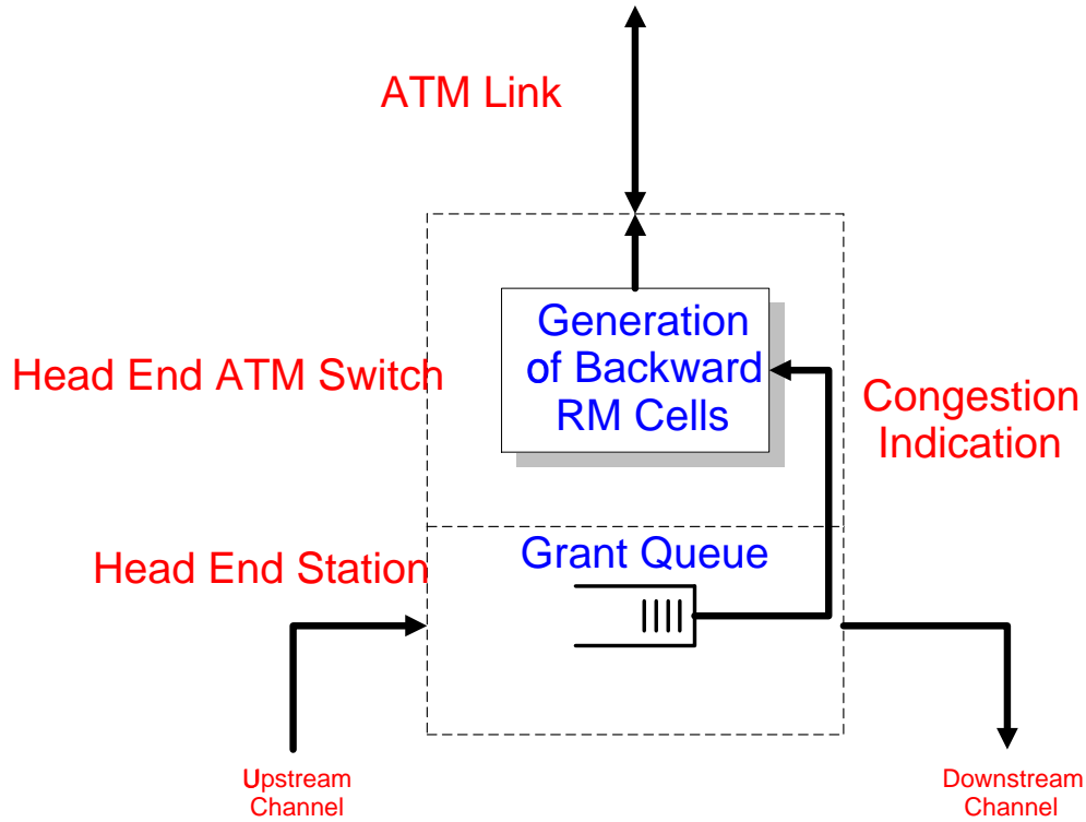
Figure 2.9: Modified Headend Station.
