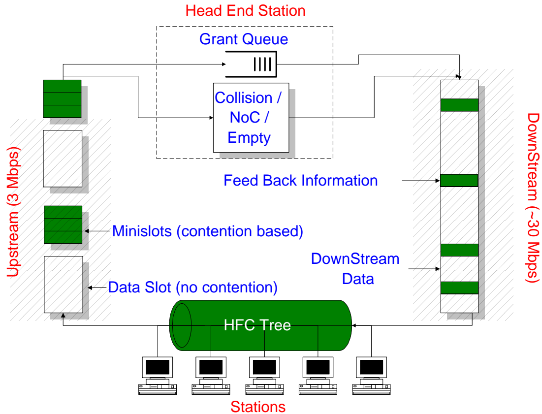
Figure 2.1: Media Access Control in HFC Networks.
