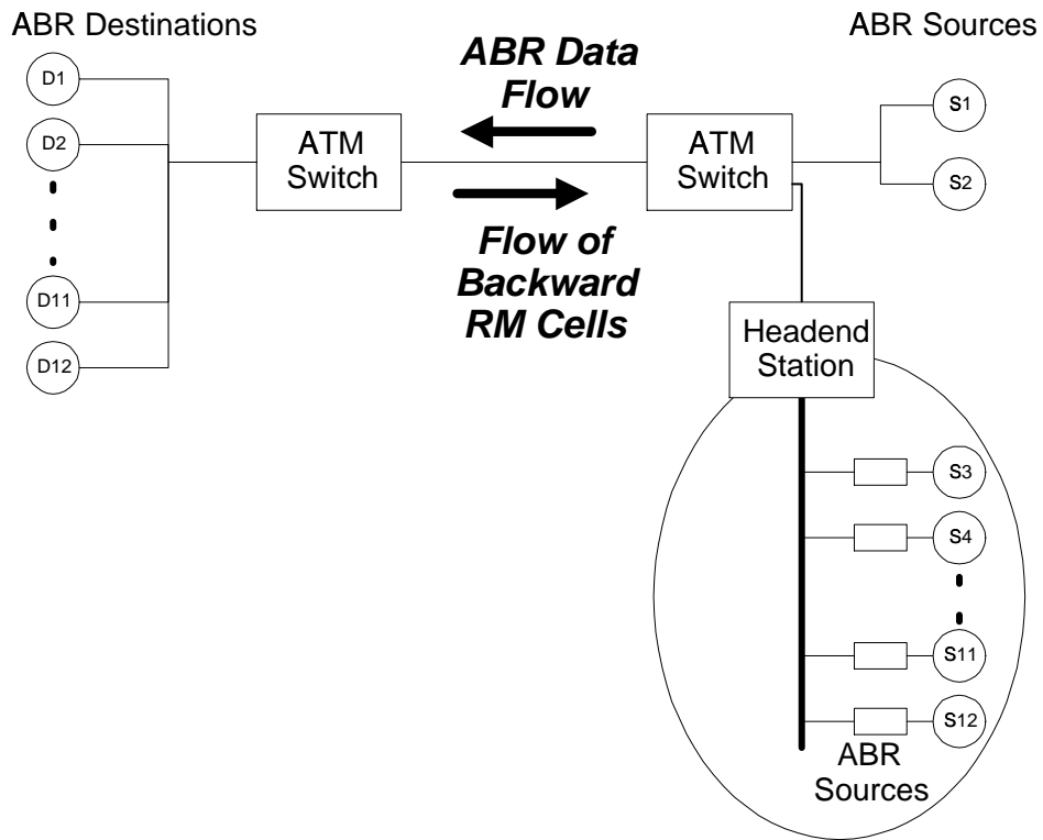
Figure 2.3: Upstream Configuration.
