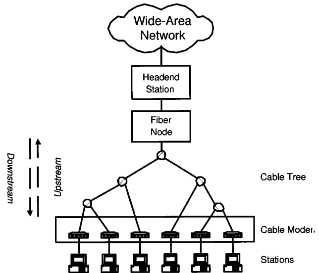
Fig. 1. HFC architecture.
